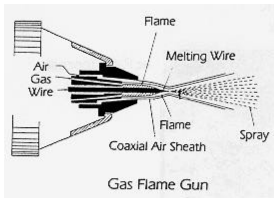
Fig. (2) Details of the Flame Spray Gun
