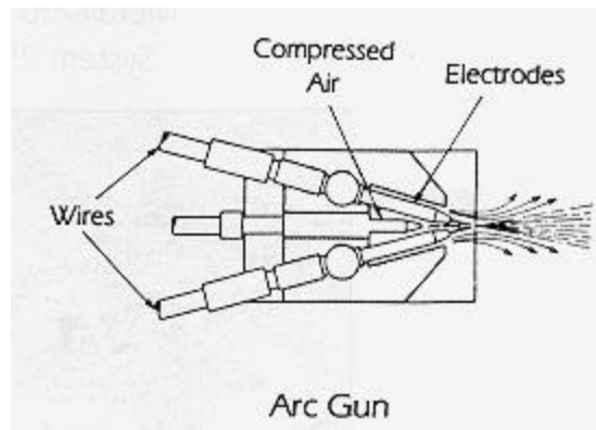
Fig. (3) Details of the Arc Spray Gun
